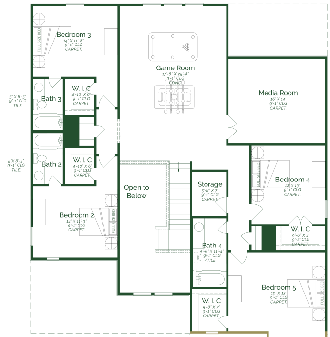
SECOND FLOOR
