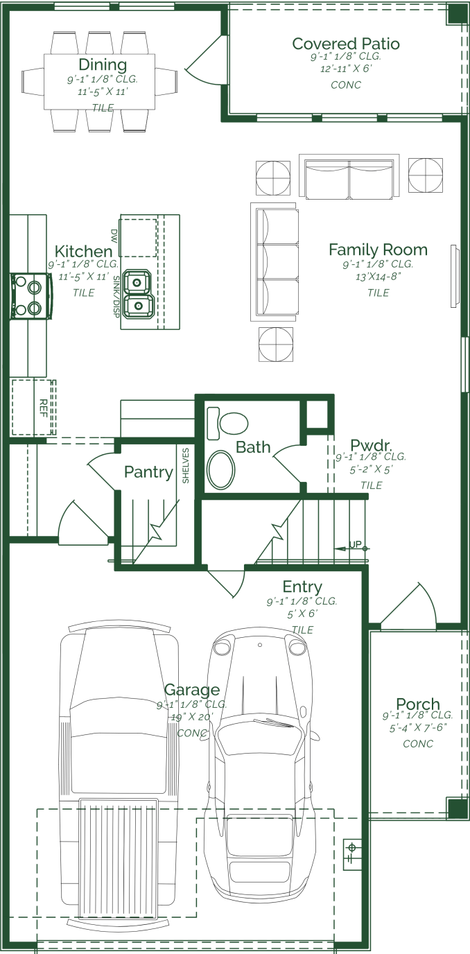
FIRST FLOOR
