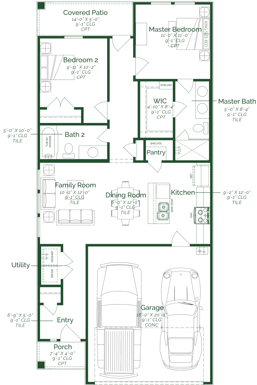
FIRST FLOOR
