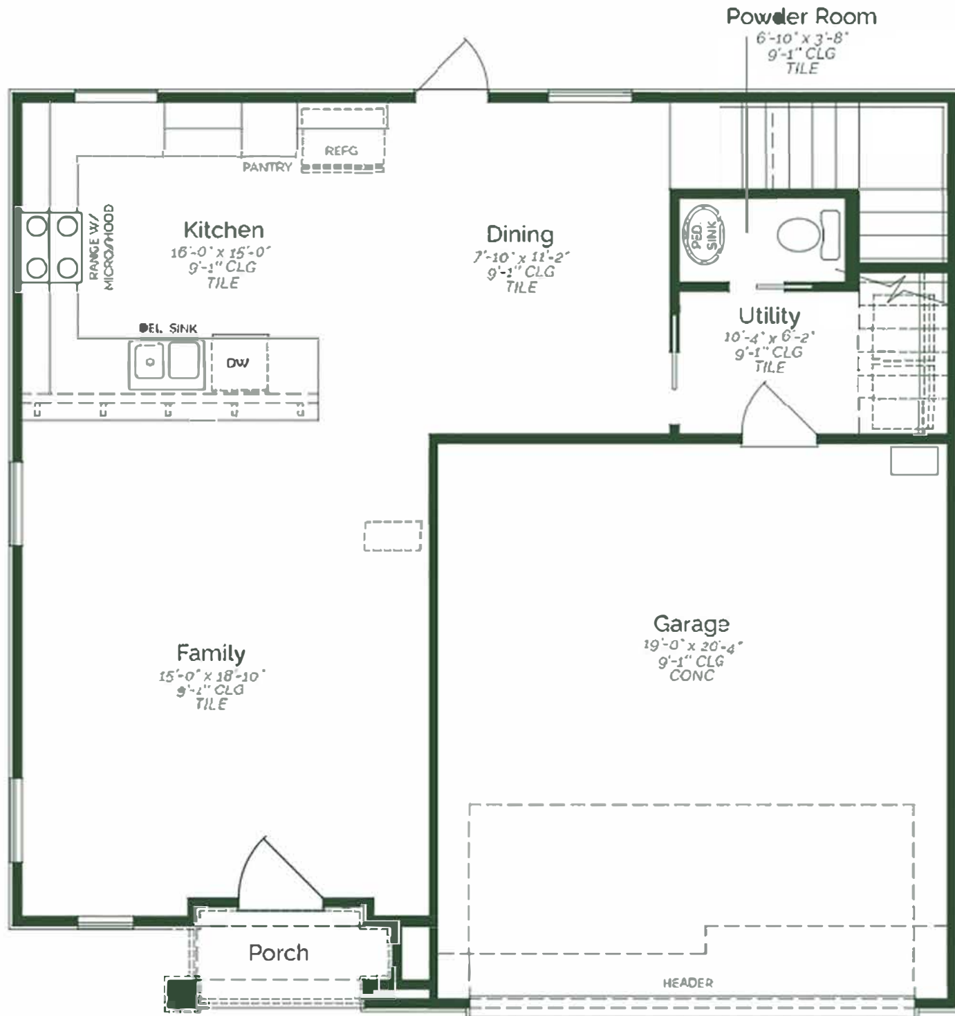
FIRST FLOOR
