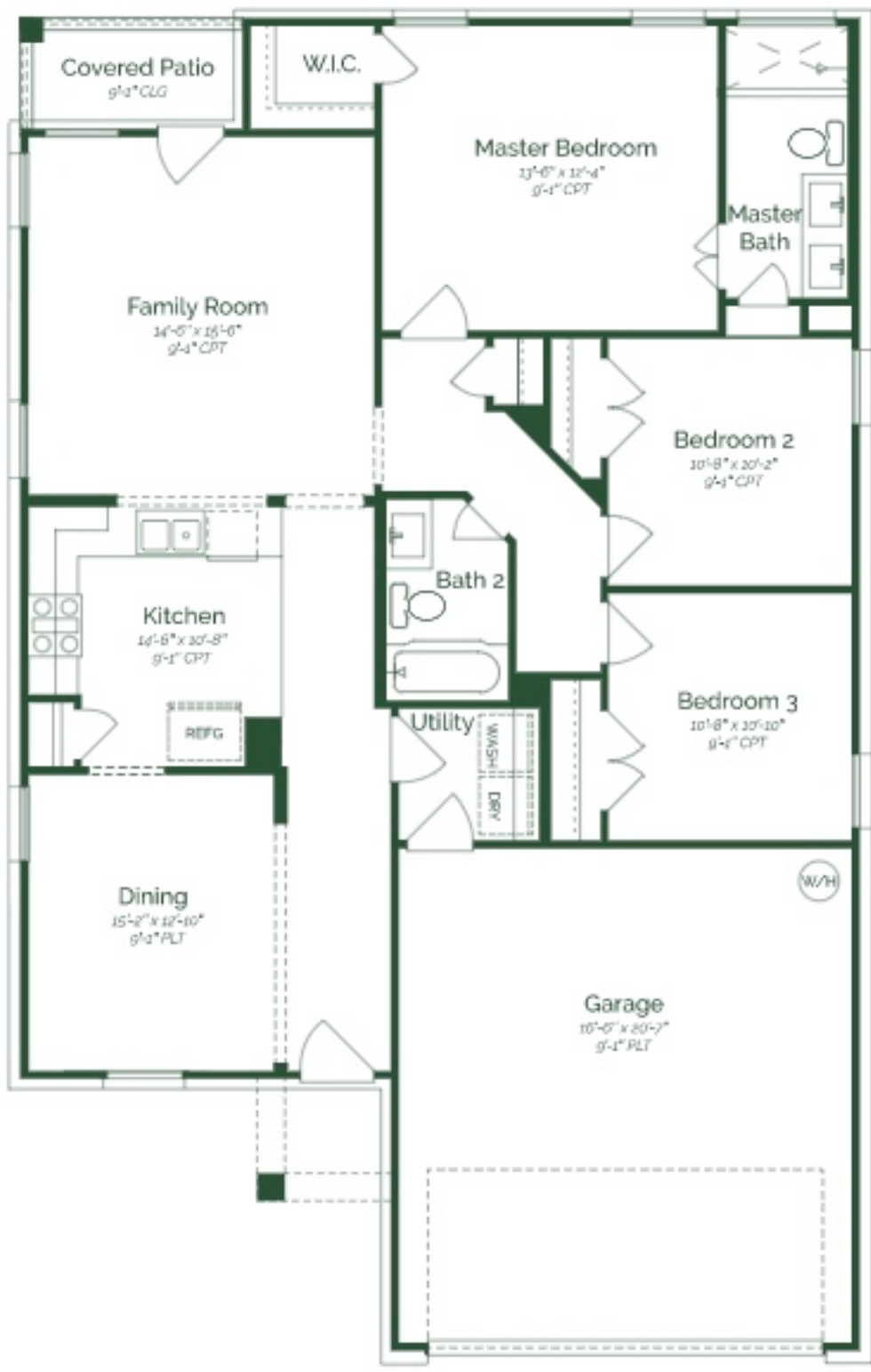
FIRST FLOOR
